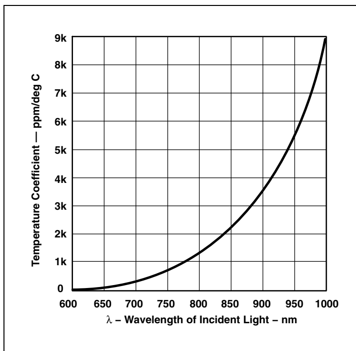
Figure 14: Photodiode Responsivity Temperature Coefficient vs. Wavelength Of Incident Light
