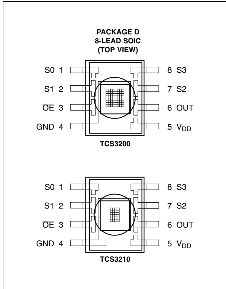
Figure 3: Pin Diagram of TCS3200/TCS3210
